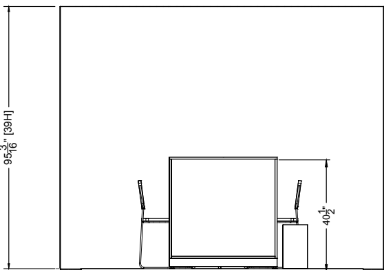
Front Elevation
