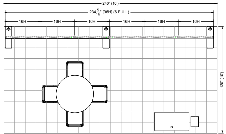
Electrical - Top View
