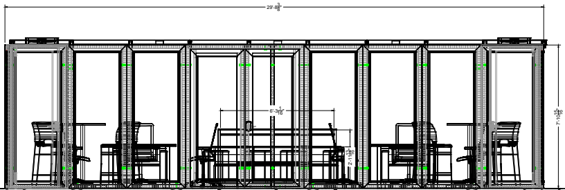
Front Elevation
